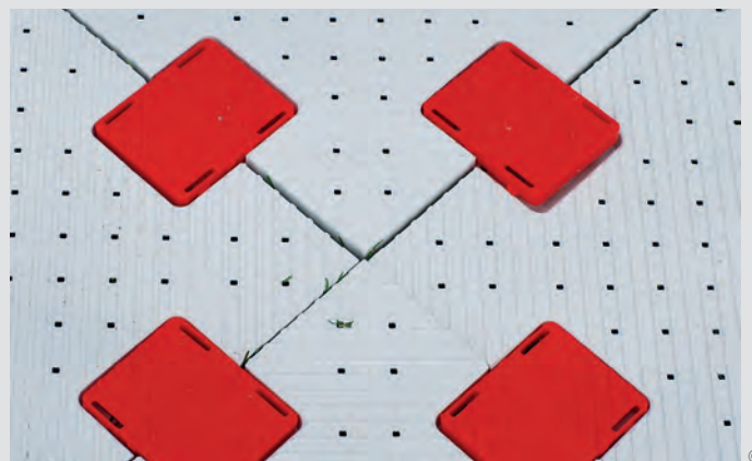
The eps Pro panels are connected by a patented locking clip system
